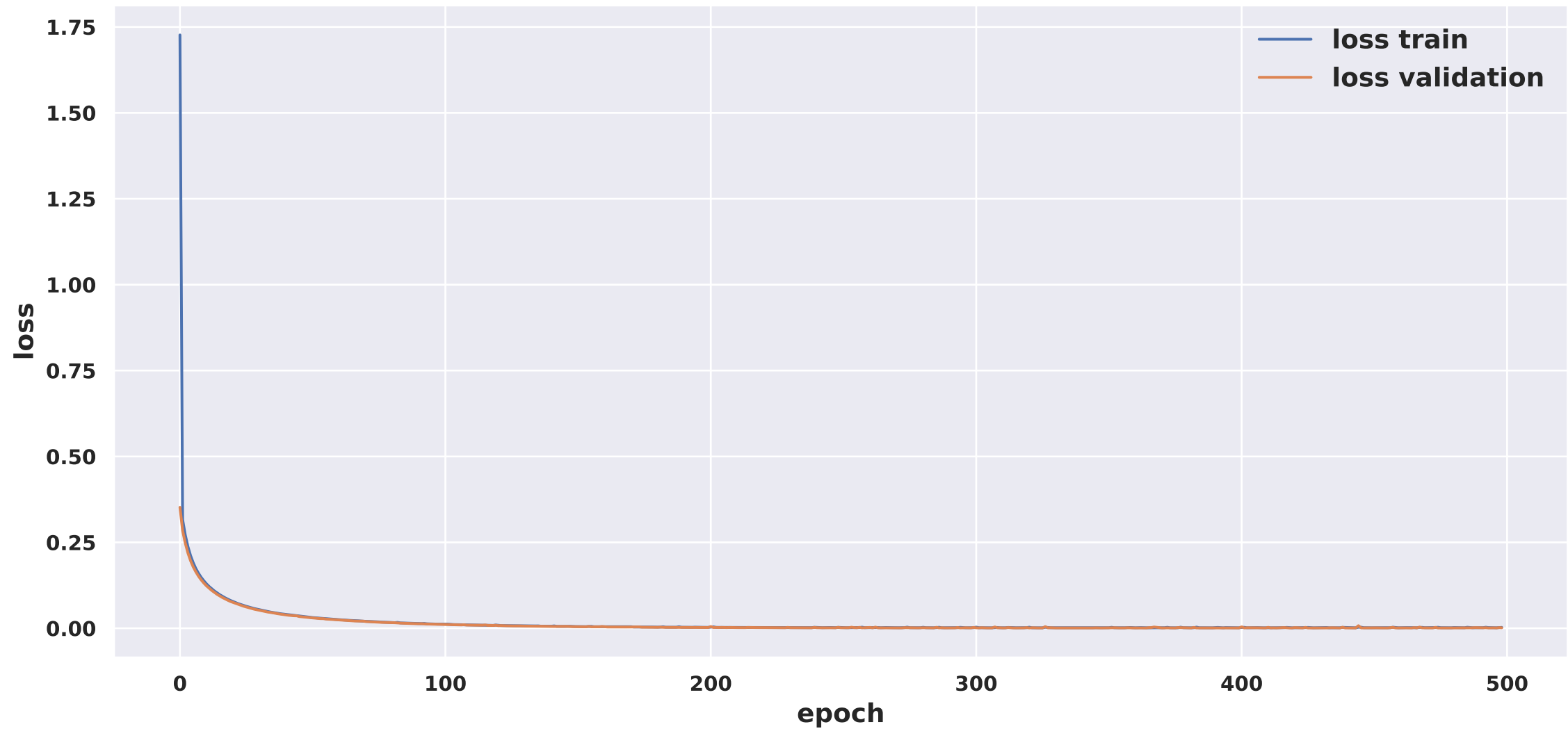
Adani Enterprises - Bi-LSTM Train and Validation Loss
